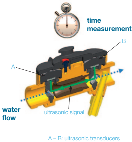
A – B: ultrasonic transducers
