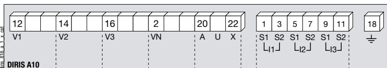
DIRIS A10 S1 - S2: current inputs.
