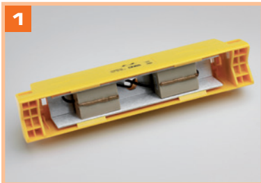
1 Guide rail and sensor assembly showing grease applied
