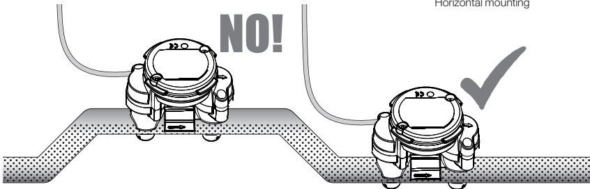
Horizontal mounting
