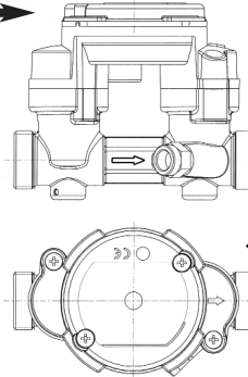
Horizontal mounting
