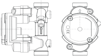
Vertical mounting
